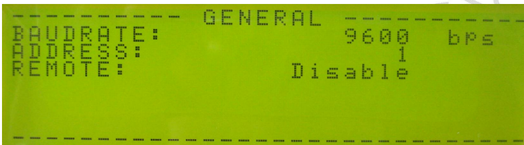
Figure 8-9 Page of GERNERAL Menu
