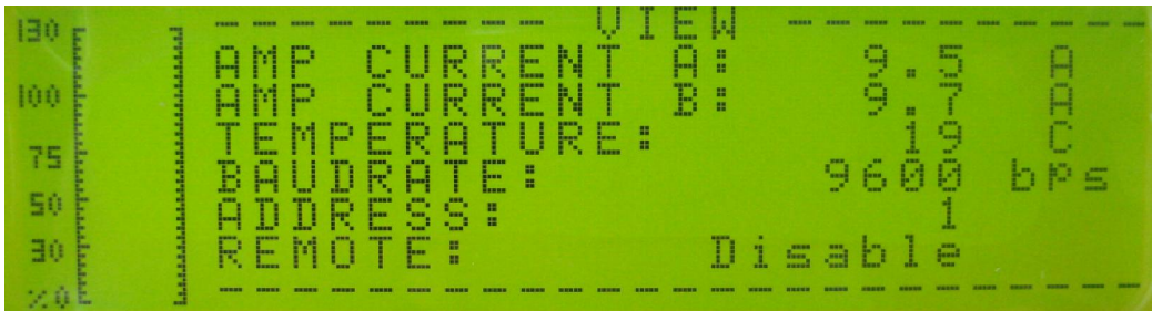
Figure 8-4 Page of VIEW
