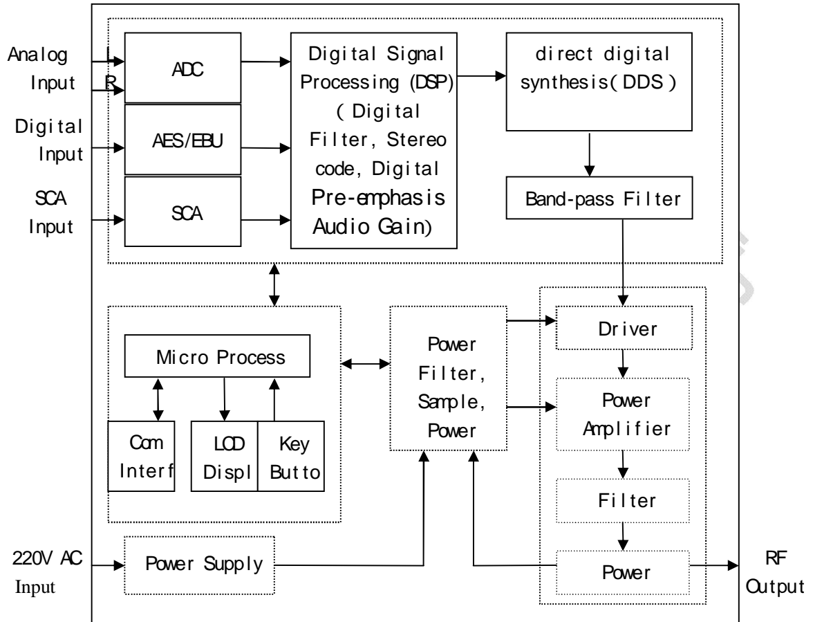
Figure 3-1 CZH618F-2000C 2000W transmitter structure and function
