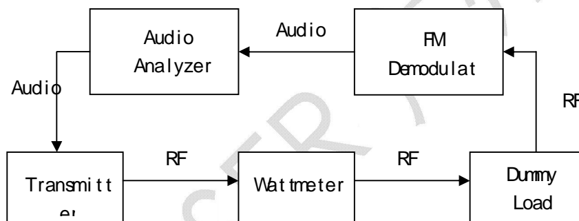
Figure 4-1 connecting for audio analyze
